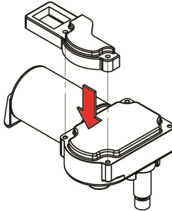
USE 4mm SCREWS TO SECURE BRACKET
